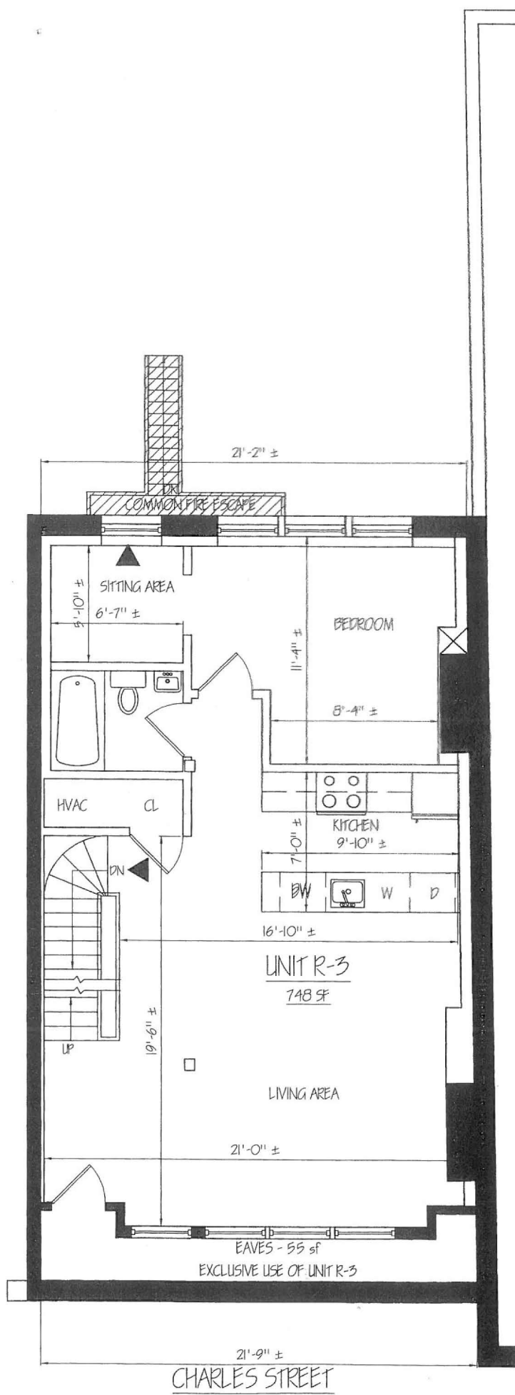
3 FOURTH FLOOR PLAN 1/4" = 1'-0"
