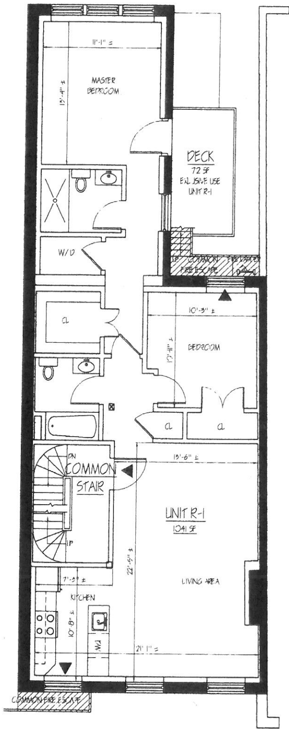
3 AS BUILT 2nd FLOOR PLAN 1/4" = 1'-0"
