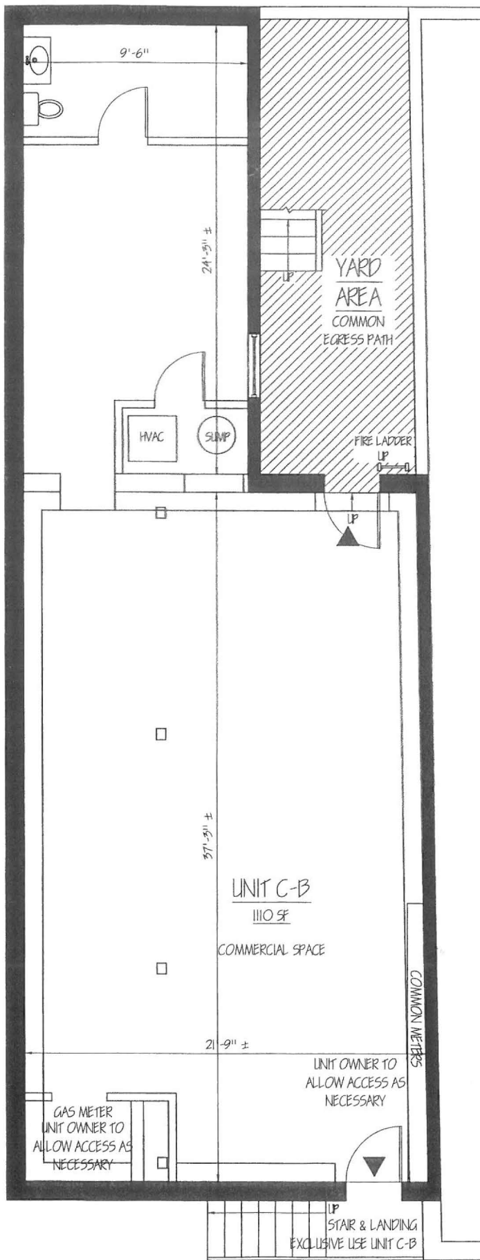
2 BASEMENT FLOOR PLAN 1/4"=1'-0"
