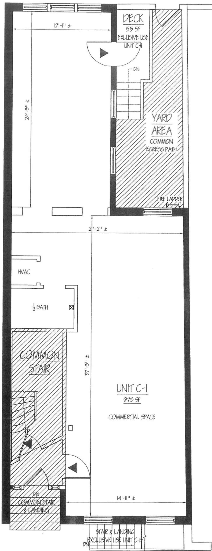
3 FIRST FLOOR PLAN 1/4"=1'-0"
